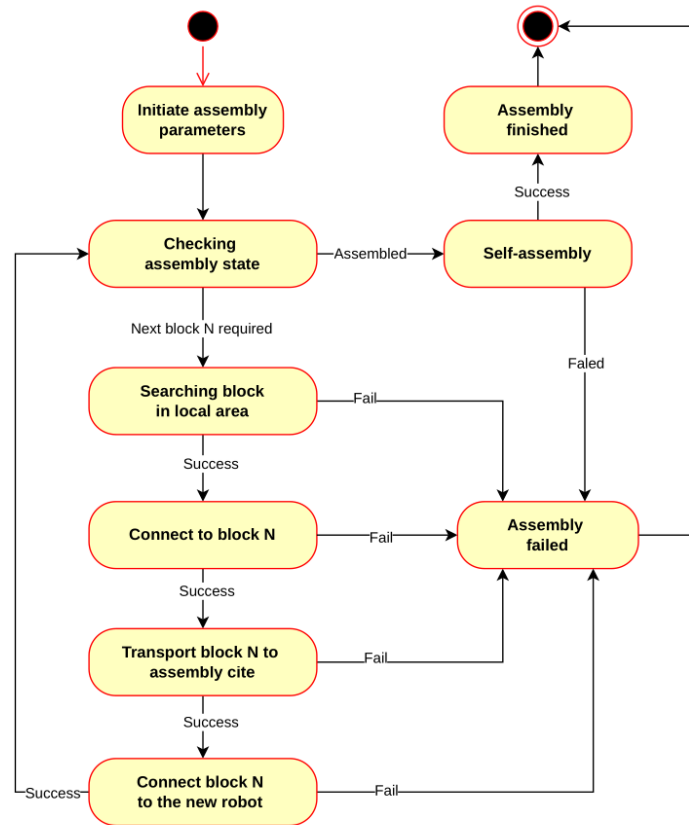
Figure 5.3: Local assembly process without model checking
